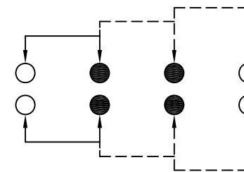
SCHEMATIC (NON-SHORTING)
